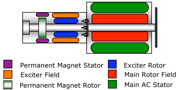
PMG Excited Generator
