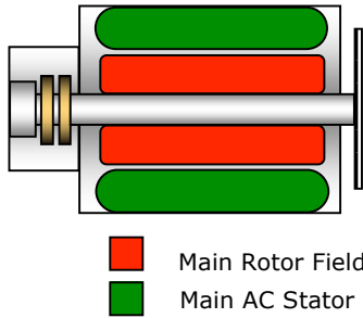
Slip Ring Fed Rotor
