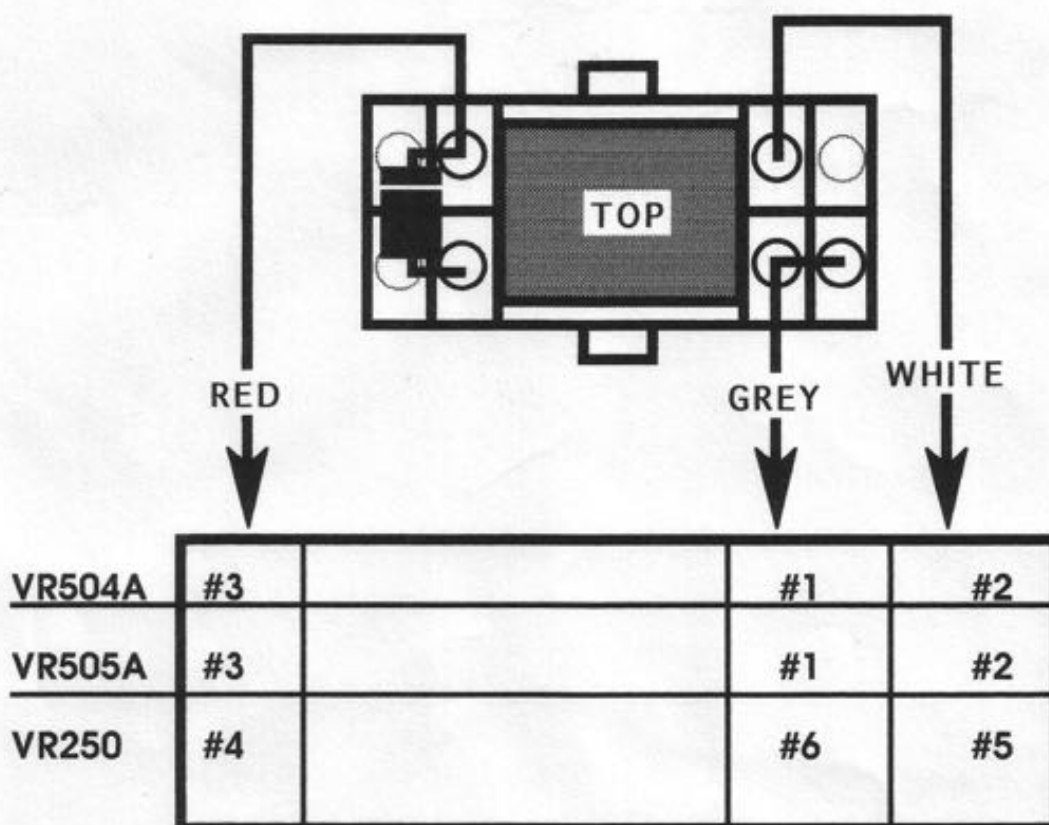
Terminal board connections
