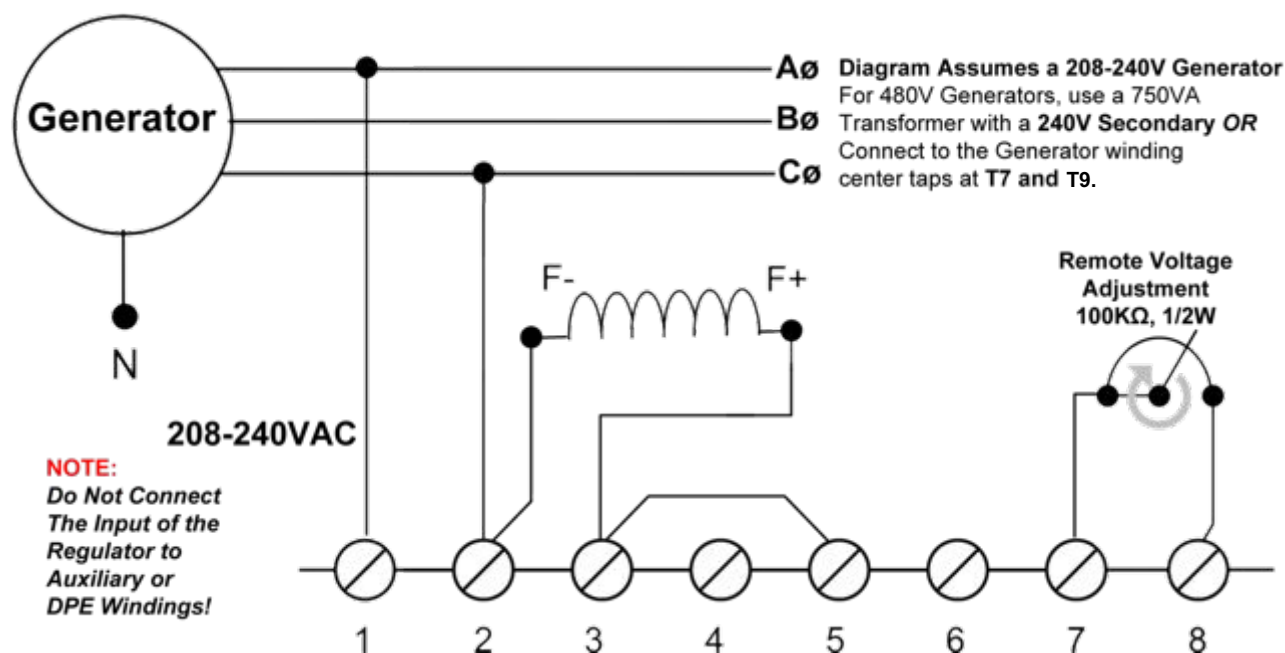
XR500C-400 Universal Voltage Regulator
